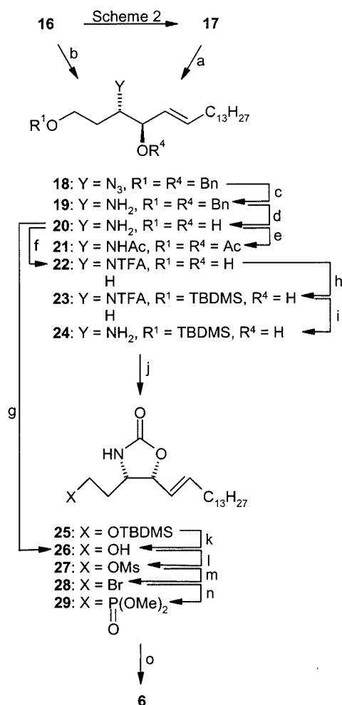
Scheme 3. Reagents and conditions: (a) NaN 3 , DMF, 100 °C, 5 h (82%); (b) PPh 3 , DIAD, Zn(N 3 ) 2 ·Pyr 2 , Tol, 50 °C (50%); (c) PPh 3 , Pyr/H 2 O, 50 °C, 15 h (80%); (d) Li, NH 3 (l), THF, –78 °C → –45 °C, 3 h, (52%); (e) Ac 2 O, Pyr, room temp., 30 h, (87%); (f) CF 3 COSEt, NEt 3 , MeOH, room temp., 4 h (90%); (g) CDI, THF, –78 °C (byprod. 10–15%); (h) TBDMS–Cl, Pyr, CH 2 Cl 2 , room temp., 1.5 h (89%); (i) K 2 CO 3 , MeOH/H 2 O, refl. 1 h (75%); (j) CDI, THF, room temp., 5 h (85%); (k) pTsOH, THF/H 2 O, room temp., 30 h (93%); (l) MeSO 2 Cl, NEt 3 , CH 2 Cl 2 , room temp., 3 h (99%); (m) LiBr, THF, 60 °C, 60 h (93%); (n) (MeO) 3 P, refl., 50 h (97%); (o) LiOH, EtOH/H 2 O, refl., 3 d (31%).
