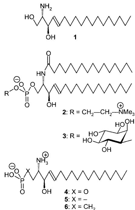
Scheme 1. Structure of compounds 1–6.
