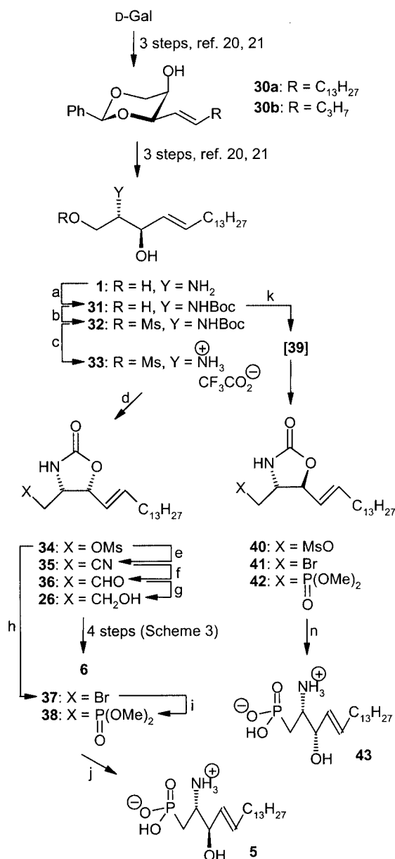
Scheme 4. Reagents and conditions: (a) Boc 2 O, NEt 3 , dioxane/H 2 O, room temp., 30 min (97%); (b) MsCl, Pyr, room temp., 15 min (71%); (c) TFA, CH 2 Cl 2 , room temp., 30 min (qu); (d) CDI, THF, room temp., 20 h (76%); (e) KCN, TEG, 60 °C, 5 h (79%); (f) DIBAH, Tol, -20 °C, 2 h (77%); (g) NaBH 4 , MeOH, room temp., 30 min (95%); (h) LiBr, THF, 60 °C, 24 h (98%); (i) P(OMe) 3 , refl., 50 h (95%); (j) LiOH, EtOH/H 2 O, room temp., 5 h (80%); (k) MeSO 2 Cl, Pyr, room temp., 1.5 h (71%); (l) LiBr, THF, 50 °C, 48 h (86%); (m) P(OMe) 3 , refl., 50 h (96%); (n) LiOH, EtOH/H 2 O, room temp., 5 h (69%).
