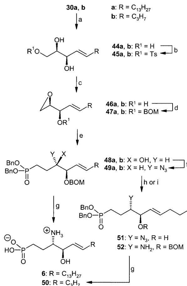
Scheme 5. Reagents and conditions: (a) Ion exchange resin: H + form, MeOH, 50 °C, 10 h (a: 61%, b: 65%); (b) p TsCl, Pyr, -15 °C, 24 h (a: 72%, b: 67%); (c) NaH, THF/DMSO, room temp., 2 h (a: 73%, b: 64%); (d) BOMCl, DIPEA, CH 2 Cl 2 , room temp., 48 h (a: 95%, b: 95%); (e) MePO(OBn) 2 , BuLi, THF, -80 °C, 2 h; BF 3 ·OEt 2 , 2 h (a, b ~ 90%); (f) Zn(N 3 ) 2 ·Pyr 2 , PPh 3 , DIAD, Tol, 50 °C, 5 h (a: 83%, b: 83%); (g) Na, NH 3 (l), -60 °C, 5 min (qu); (h) p TsOH, t BuOH, refl., 6 h (47%); (i) PPh 3 , H 2 O, 50 °C, 16 h (73%).
