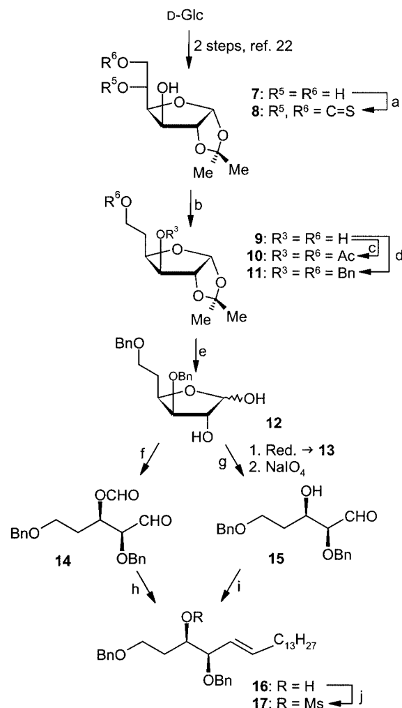
Scheme 2. Reagents and conditions: (a) TCDI, THF refl., 2 h (76%); (b) Bu 3 SnH, AIBN, dioxane refl., 2 h, (71%); (c) Ac 2 O, Pyr, 15 h (79%); (d) BnBr, NaH, DMF, room temp., 5 h (89%); (e) HCl in H 2 O, THF, room temp., 60 h (82%); (f) NaIO 4 , THF/H 2 O, room temp., 5 h (90%); (g) NaBH 4 , MeOH (81%); NaIO 4 , THF/H 2 O, room temp., 1 h (91%); (h) Triphenyl(tetradecyl)phosphonium bromide in Tol, PhLi and LiBr in Et 2 O, THF, -40 °C \rightarrow room temp. (39%); (i) see (h), 50% yield; (j) MeSO 2 Cl, NEt 3 , CH 2 Cl 2 , 6 h, room temp. (87%).
